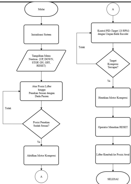
Gambar 2. Flowchart Algoritma Sistem
