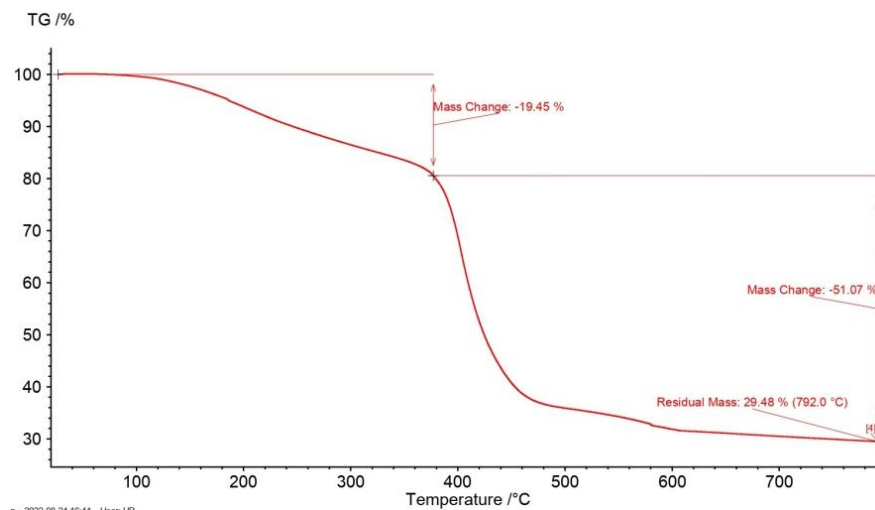
Figure 9. TG curve and \Delta m of S25%
