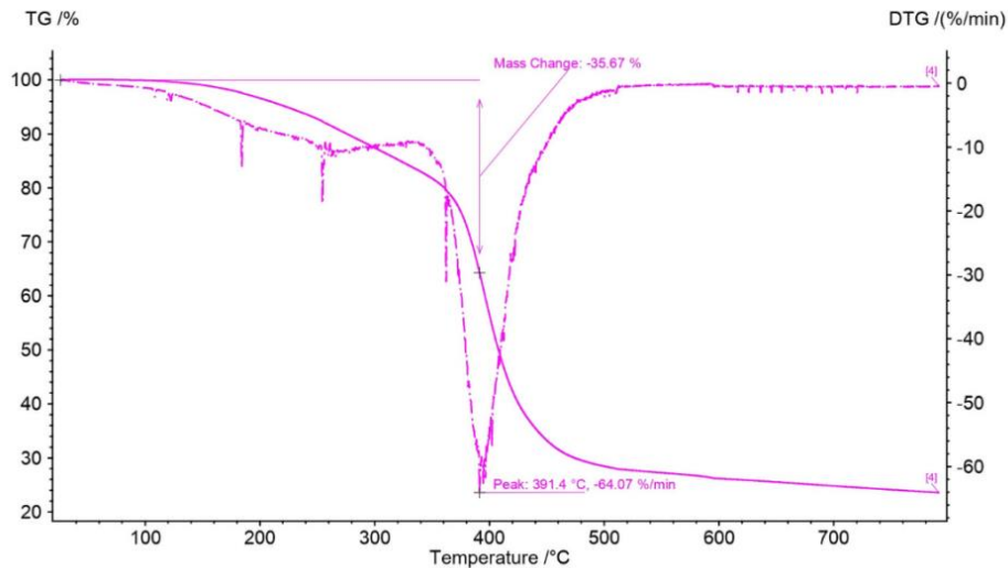
Figure 10. DTG curve of TS
