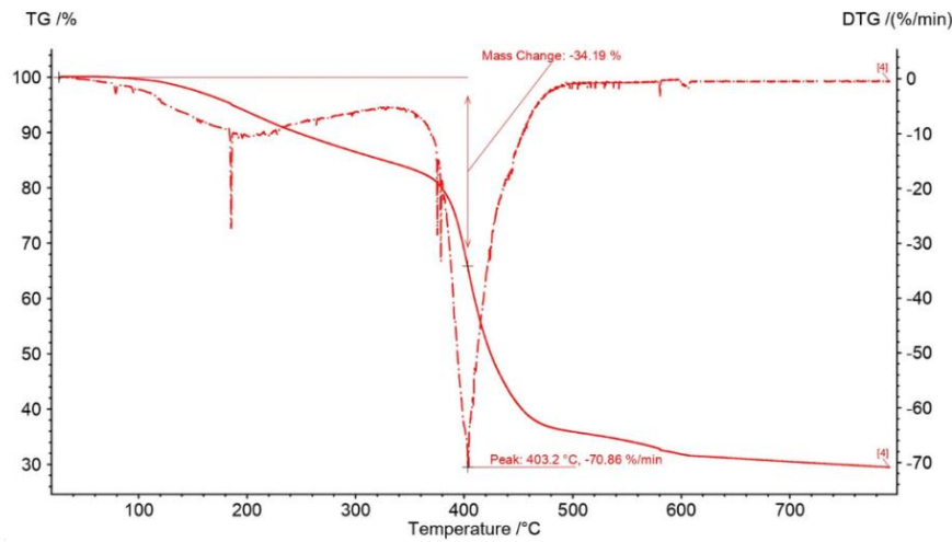
Figure 15. DTG curve of S25%
