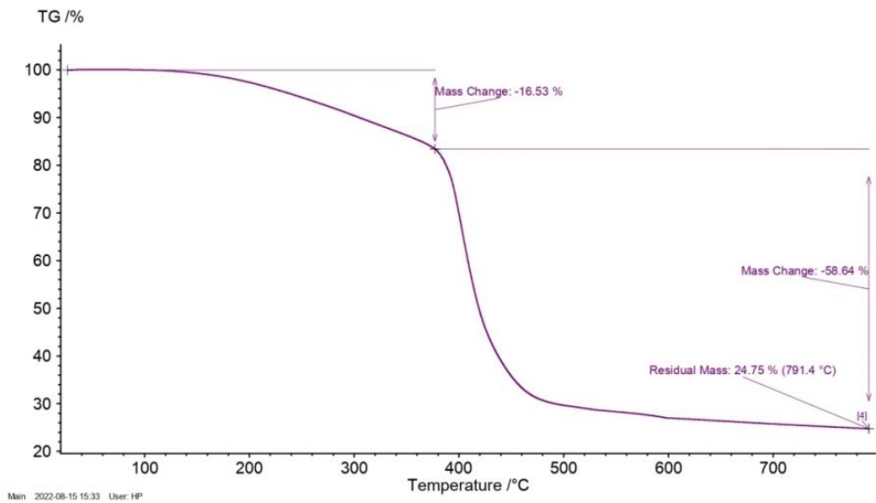
Figure 6. TG curve and \Delta m of S10%
