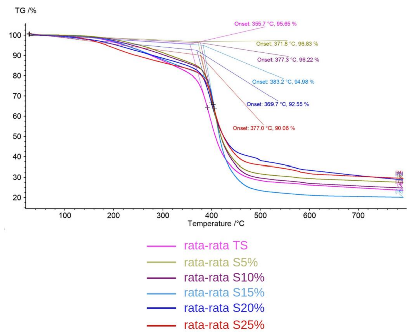
Figure 2. TG curve and extrapolated onset temperature of 6 samples
