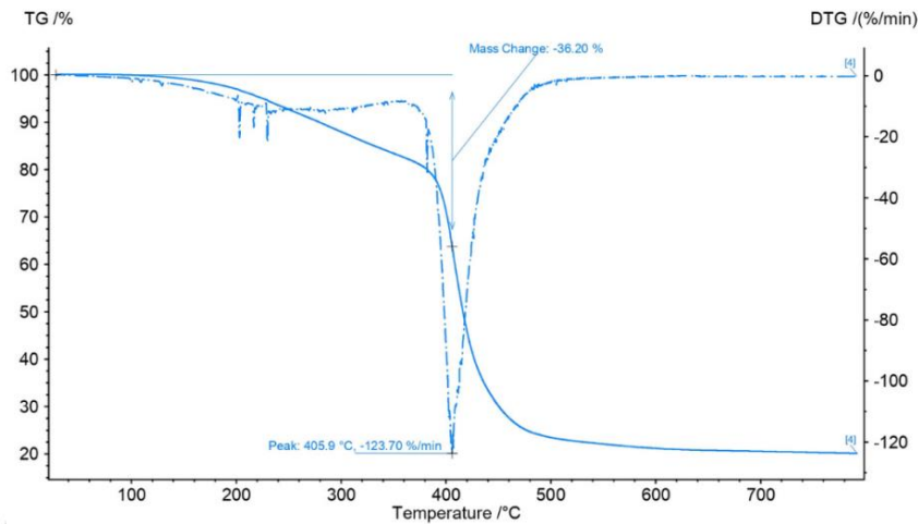
Figure 13. DTG curve of S15%
