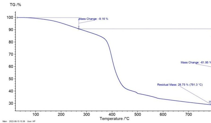
Figure 8. TG curve and \Delta m of S20%
