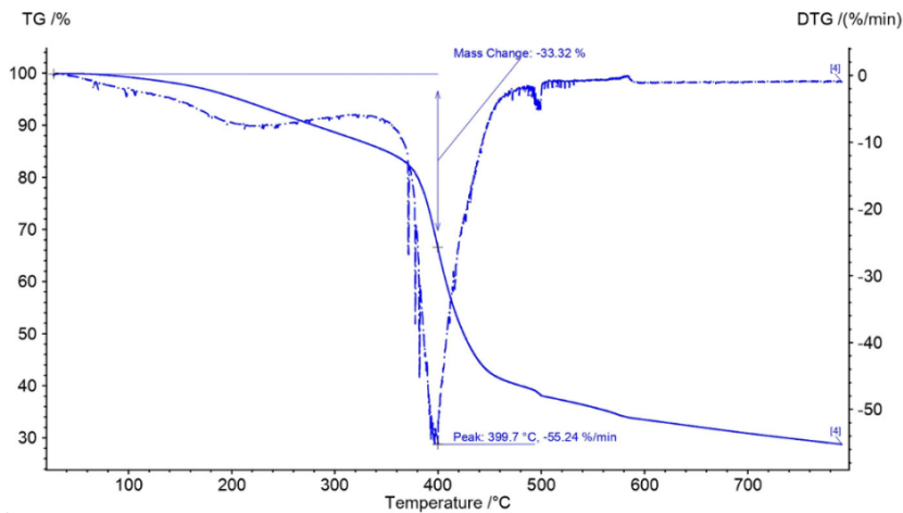
Figure 14. DTG curve of S20%
