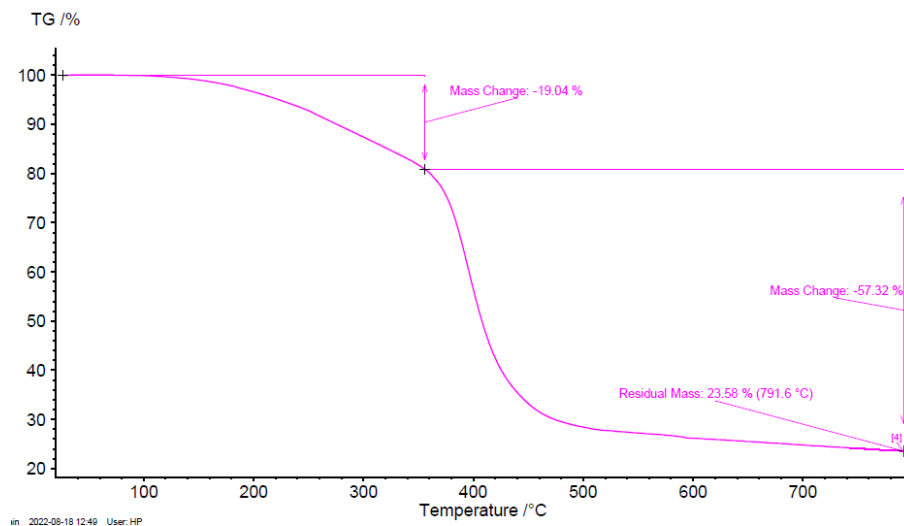
Figure 4. TG curve and \Delta m of TS
