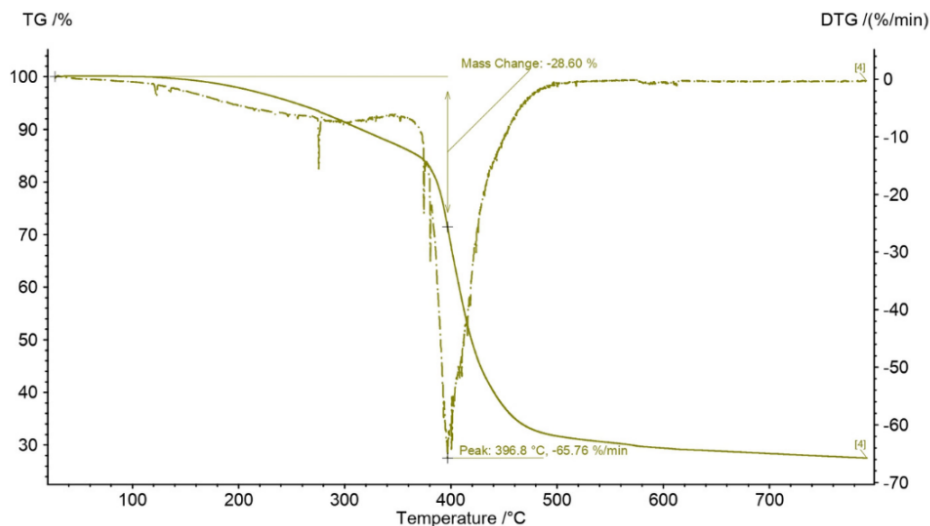
Figure 11. DTG curve of S5%
