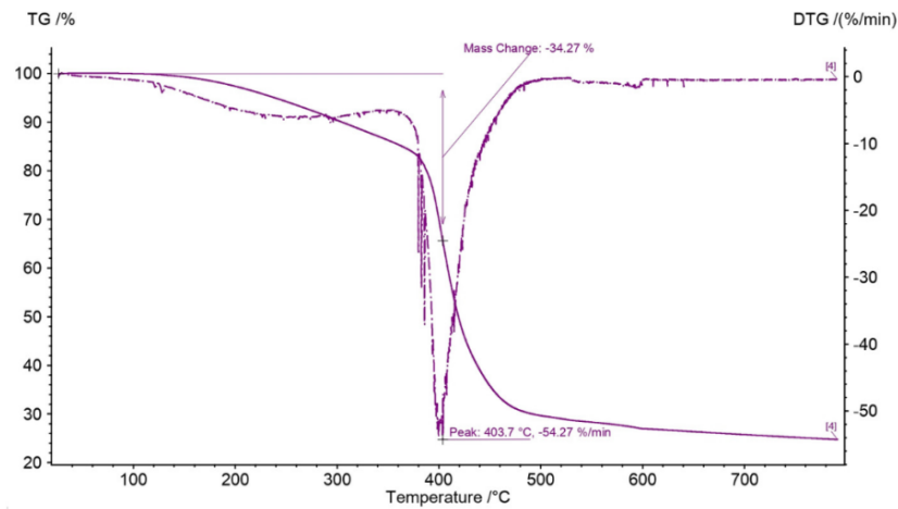
Figure 12. DTG curve of S10%
