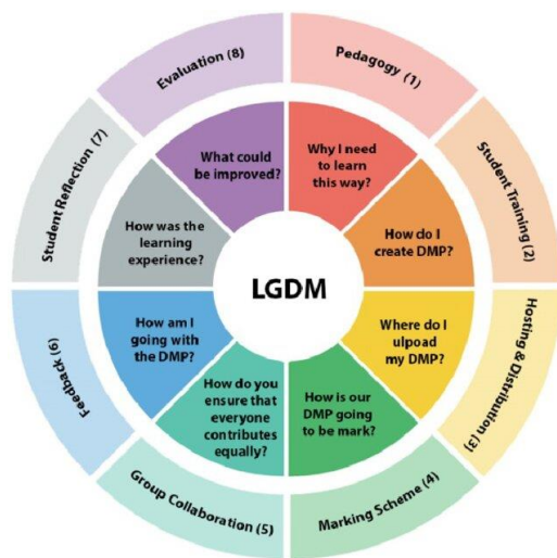
Figure 5: LGDM Framework
