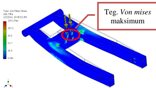
Gambar 6.1 Tegangan Von Mises Maksimum (134,135 MPa) Model A
