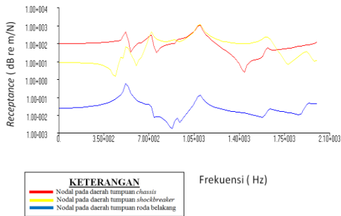
Gambar 7.13 Grafik Receptance Modulus Model C
