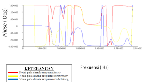
Gambar 7.14 Grafik Receptance Phase Model C
