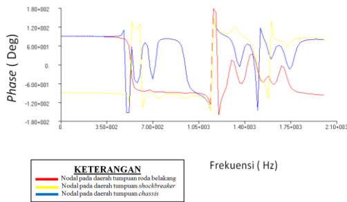
Gambar 7.4 Grafik Mobility Phase Model A
