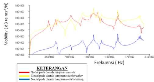
Gambar 7.21 Grafik Mobility Modulus Model D
