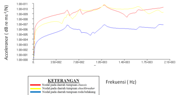
Gambar 7.17 Grafik Accelerance Modulus Model C
