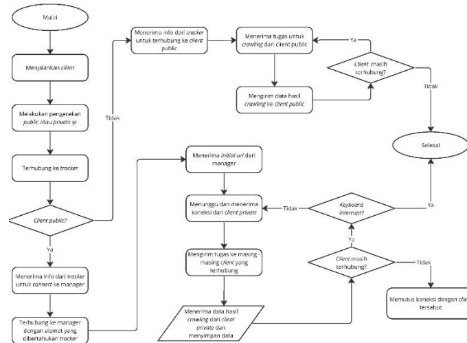
GAMBAR 8. Flowchart Client
