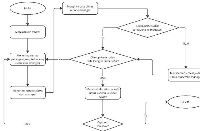
GAMBAR 6. Flowchart Tracker
