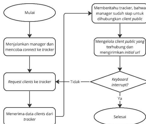
GAMBAR 7. Flowchart Manager
