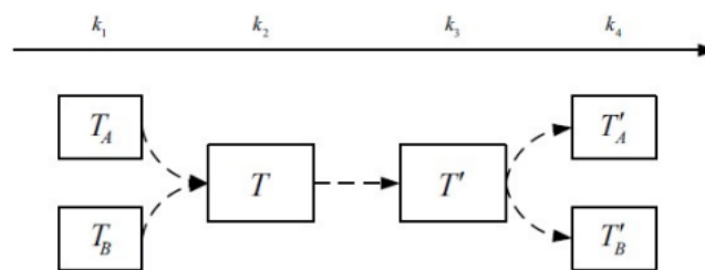
GAMBAR 1. Proses Merge dan Split
