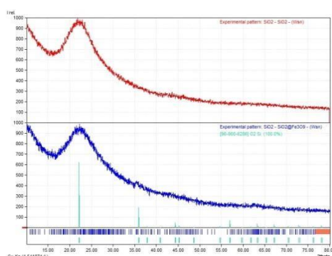
Gambar 9. Pola difraksi XRD Core-Shell \text{Fe}_3\text{O}_4\text{-SiO}_2
