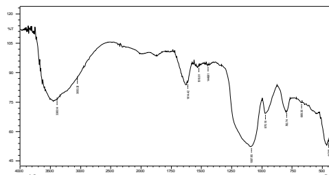
Gambar 7. Hasil FTIR Core-Shell \text{Fe}_3\text{O}_4\text{-SiO}_2
