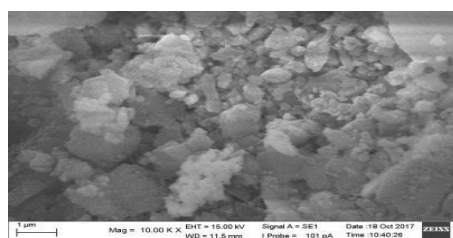
Gambar 8. Hasil SEM Core-Shell \text{Fe}_3\text{O}_4\text{-SiO}_2
