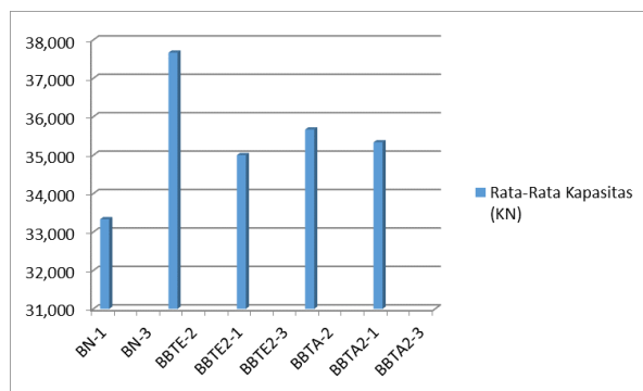
Gambar 10. Rata-Rata Beban Ultimit Balok
