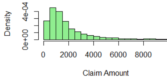
Figure 3. Histogram of claim amount (95% Data)
